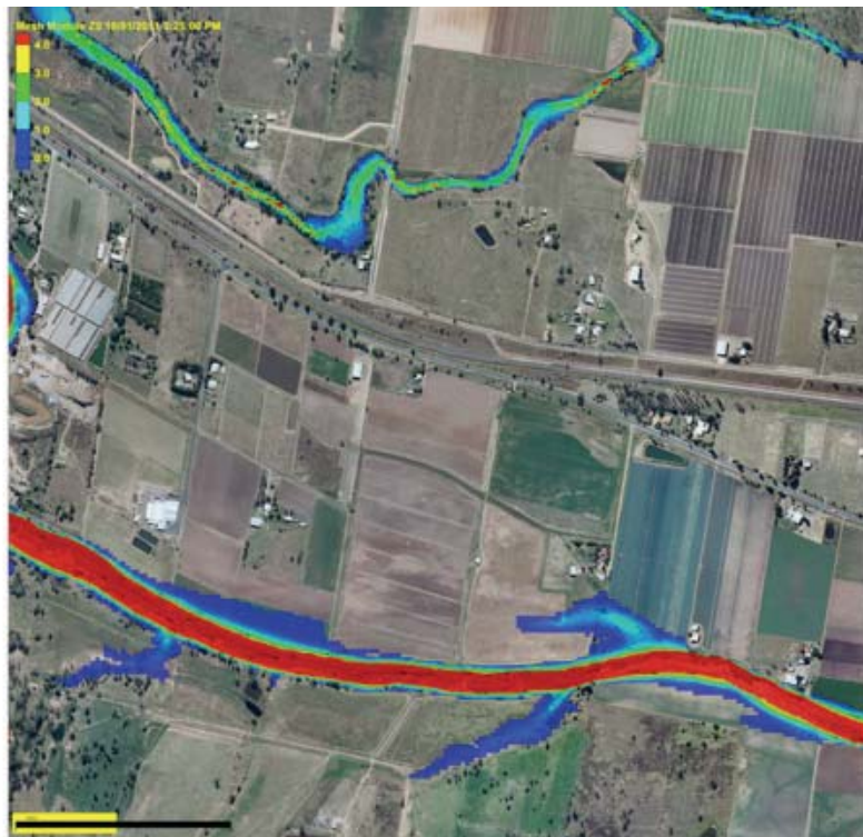
Figure 9.2 a to d – Chronology of Inundation, Western Grantham 3:25pm to 3:40pm
