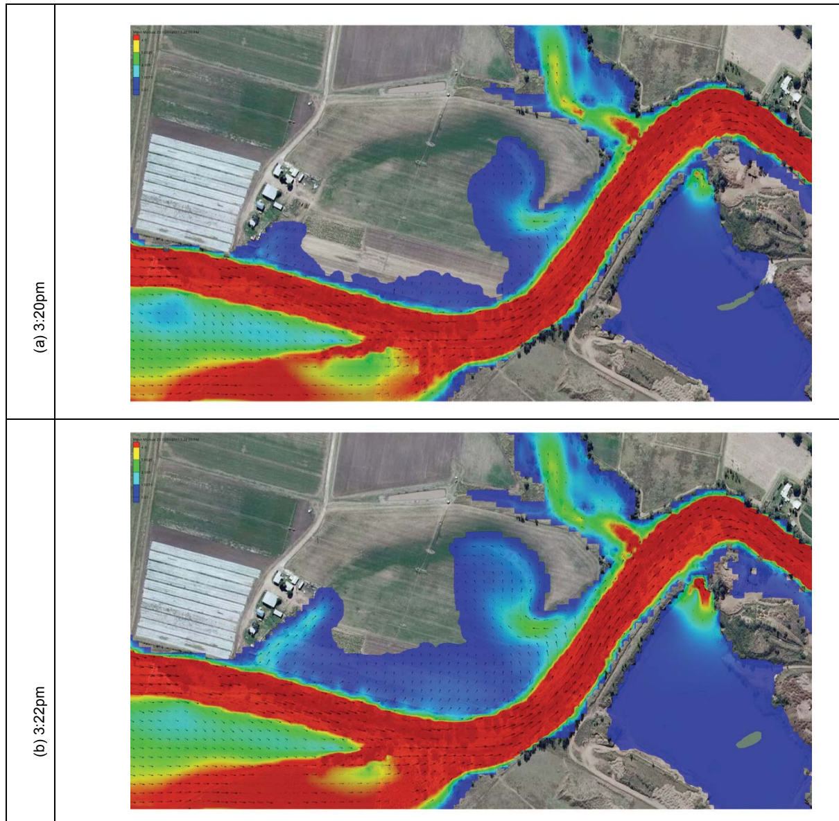
Figure 12.13 (a to b) – Flow Inundation of Oval Area Near Quarry
