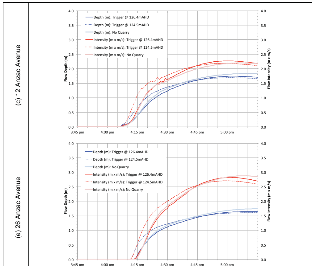
Figure 10.18 (continued) – Effect of Worst Case Quarry Levee Failure on Flow Depth and Intensity
