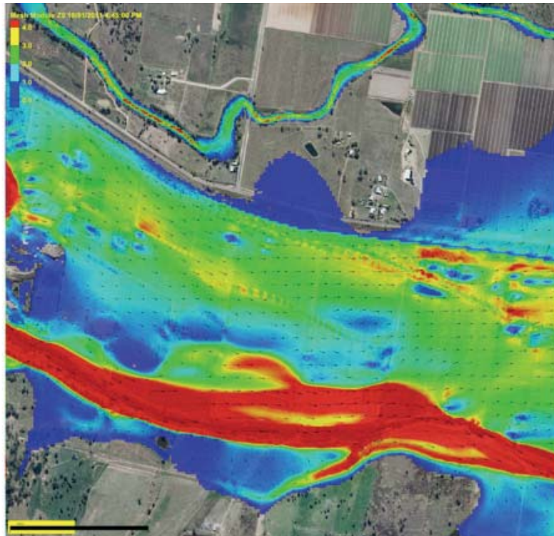
Figure 9.2 i to l – Chronology of Inundation, Western Grantham 4:25pm to 5:00pm (cont.)
