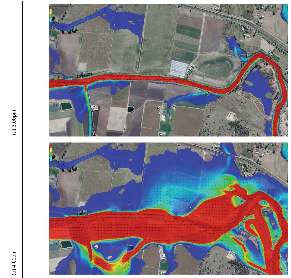
Figure 12.11 (a to b) – Flow Inundation Upstream from the Quarry
