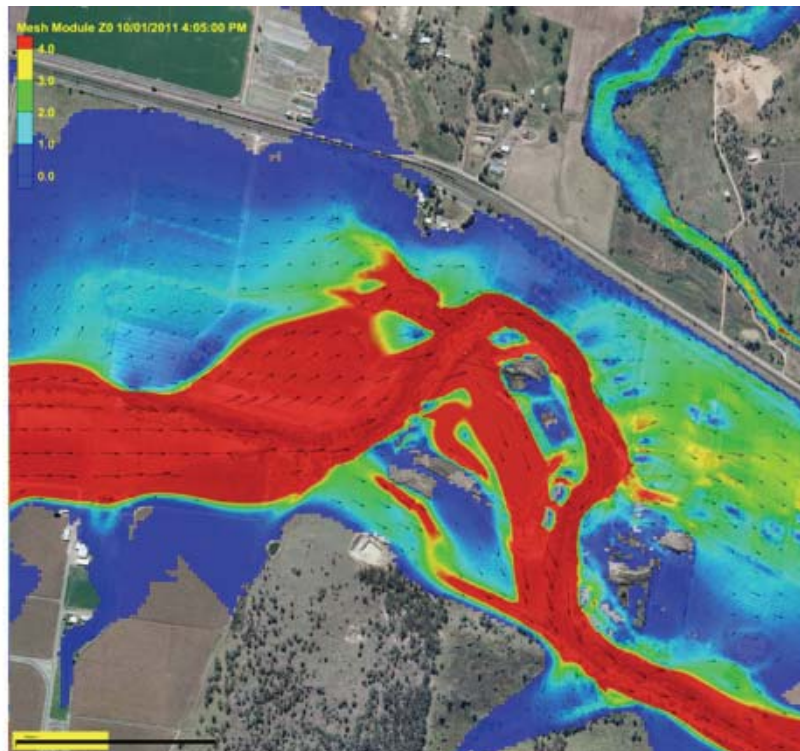
Figure 9.1 i to l – Chronology of Inundation, Quarry and Upstream 3:45pm to 4:20pm (cont.)
