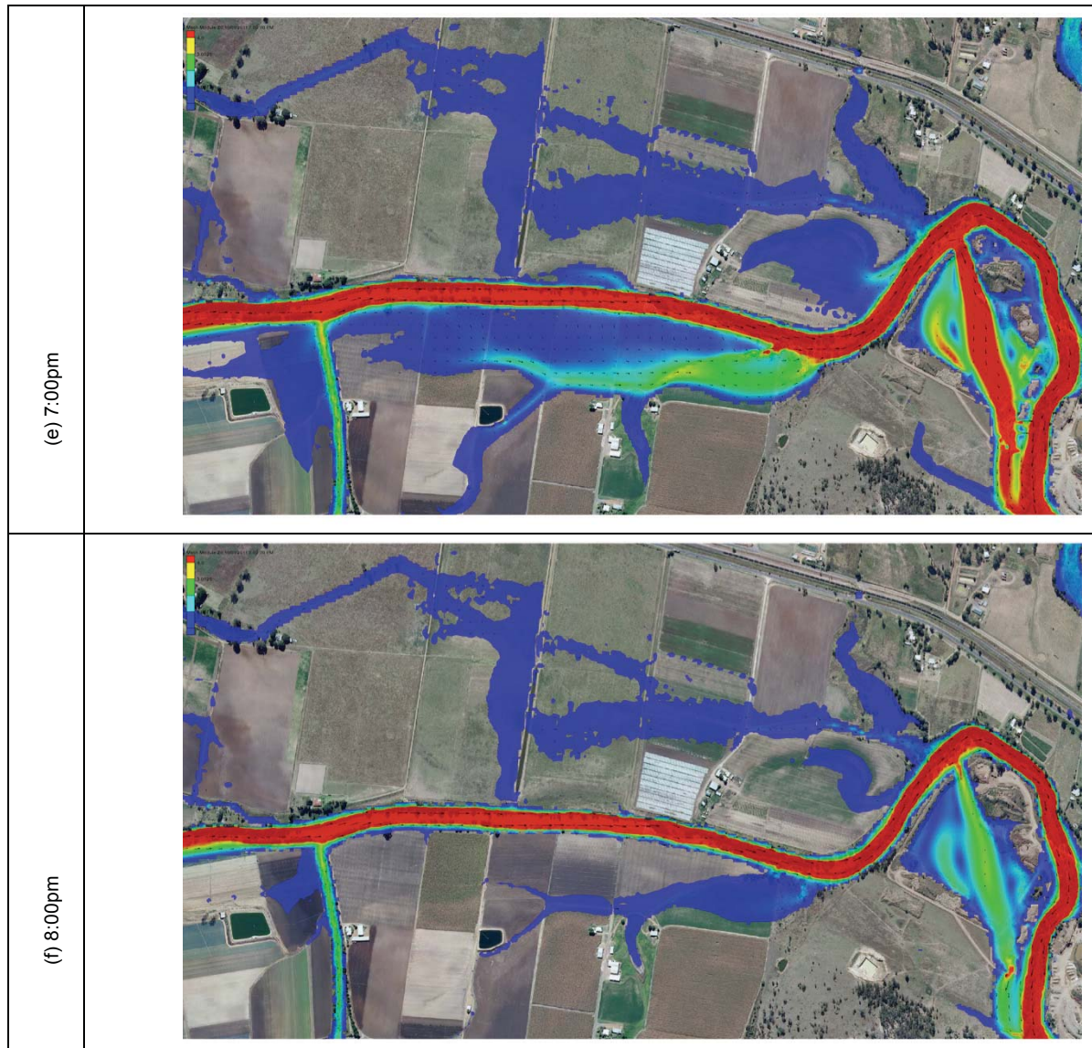
Figure 12.11 (e to f) – Flow Inundation Upstream from the Quarry
