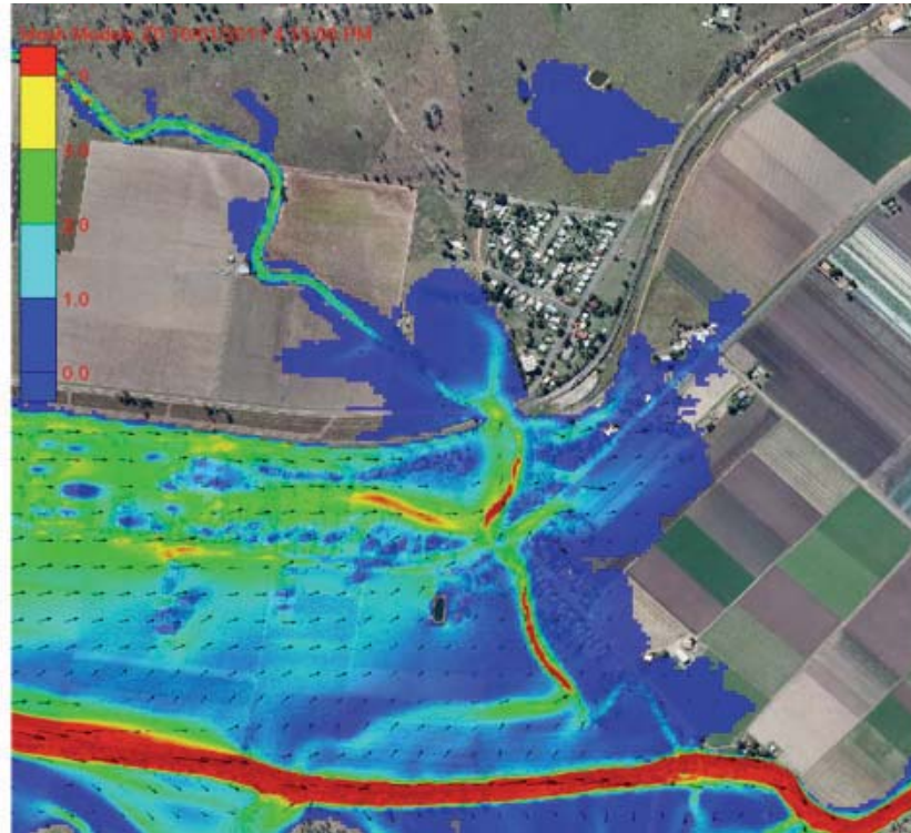
Figure 9.3 e to h – Chronology of Inundation, Central Grantham 4:05pm to 4:20pm (continued)
