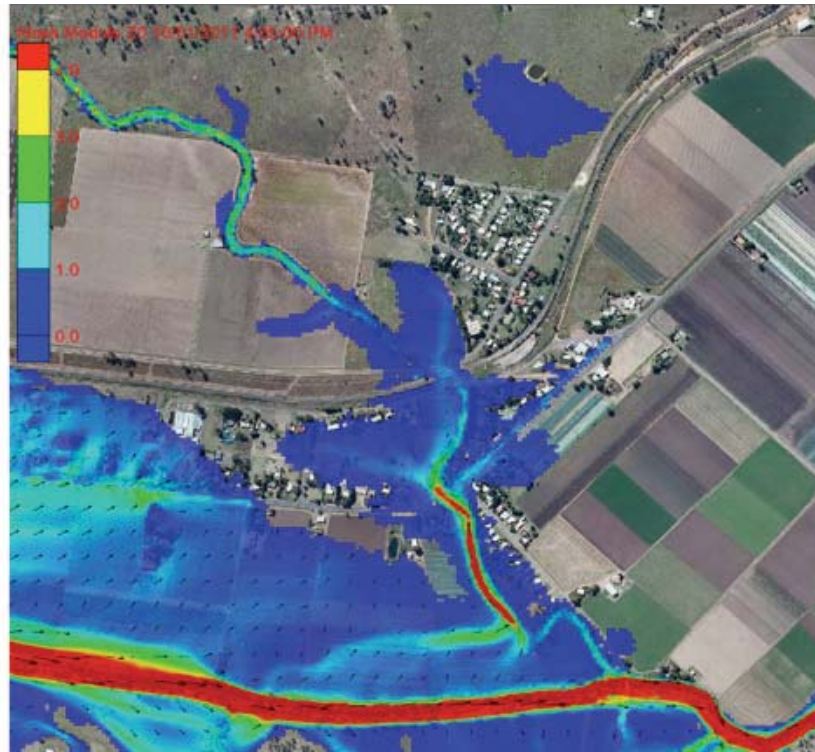
Figure 9.3 e to h – Chronology of Inundation, Central Grantham 4:05pm to 4:20pm
