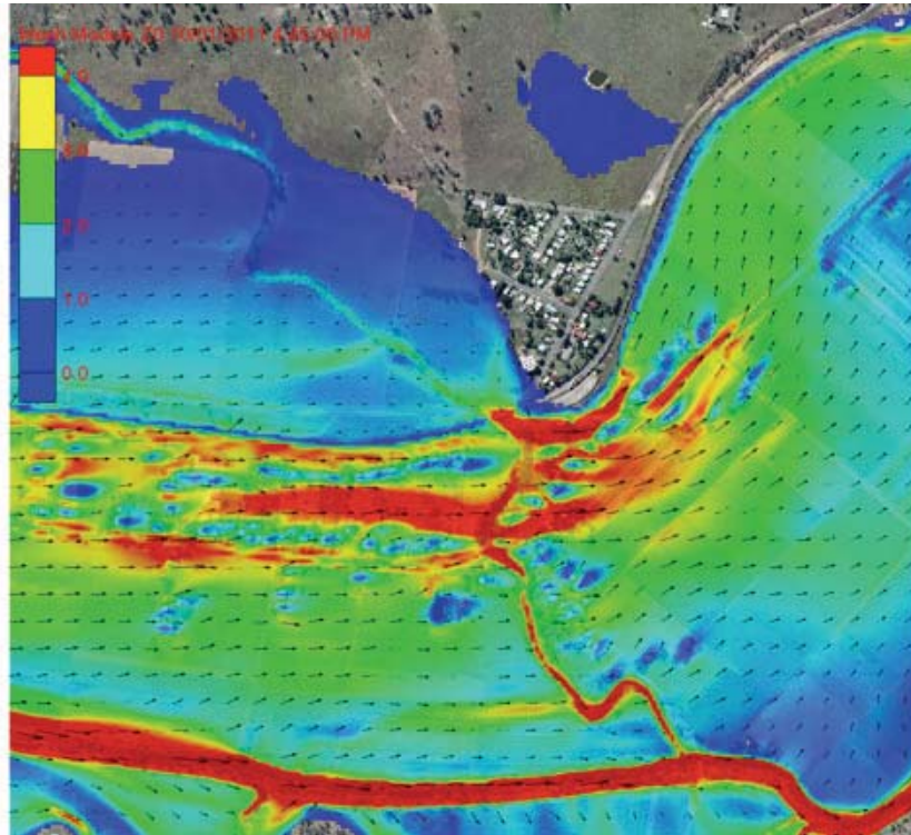
Figure 9.3 i to l – Chronology of Inundation, Eastern Grantham 4:25pm to 5:00pm (continued)
