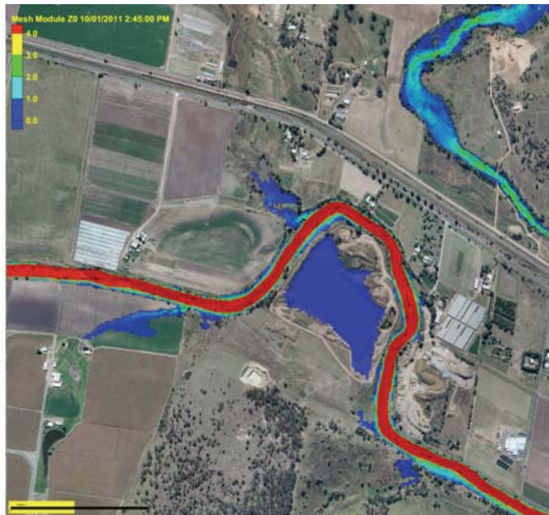
Figure 9.1 a to d – Chronology of Inundation, Quarry and Upstream 2:45pm to 3:20pm
