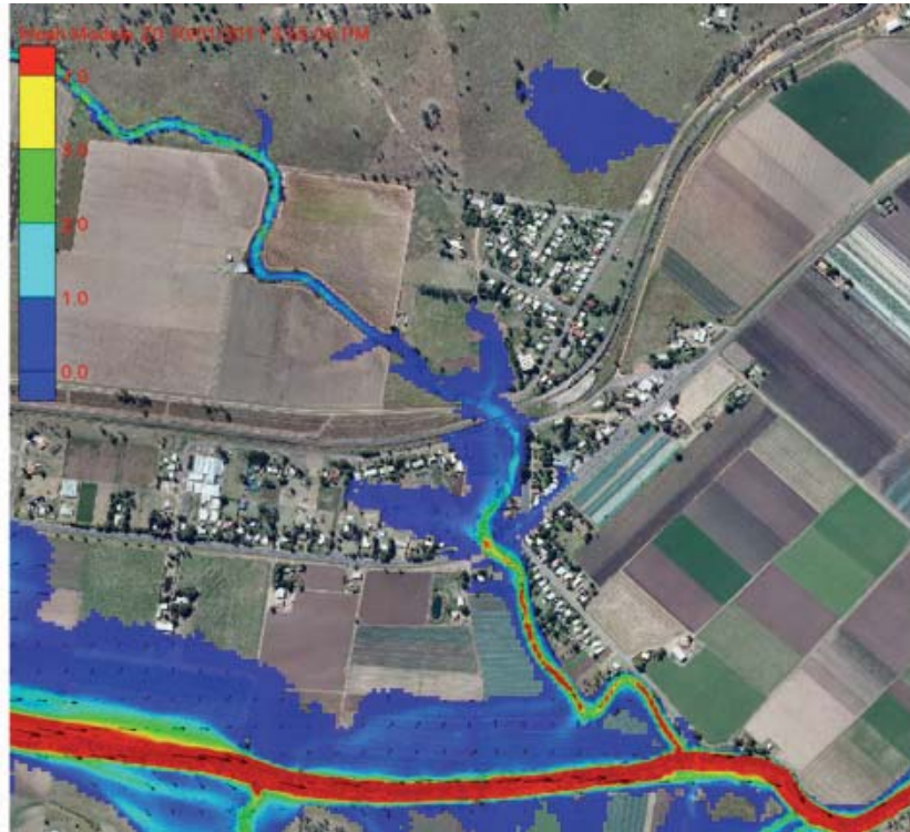
Figure 9.3 a to d – Chronology of Inundation, Central Grantham 3:25pm to 3:40pm (continued)
