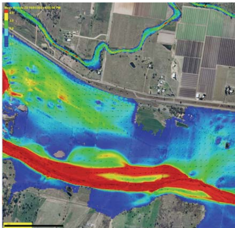
Figure 9.2 e to h – Chronology of Inundation, Western Grantham 4:05pm to 4:20pm
