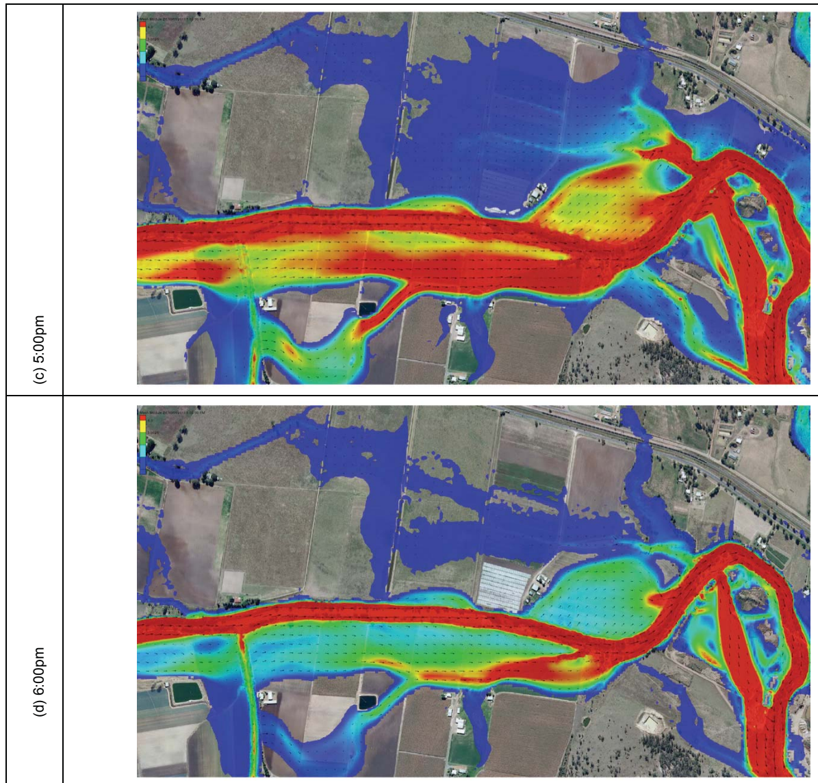
Figure 12.11 (c to d) – Flow Inundation Upstream from the Quarry
