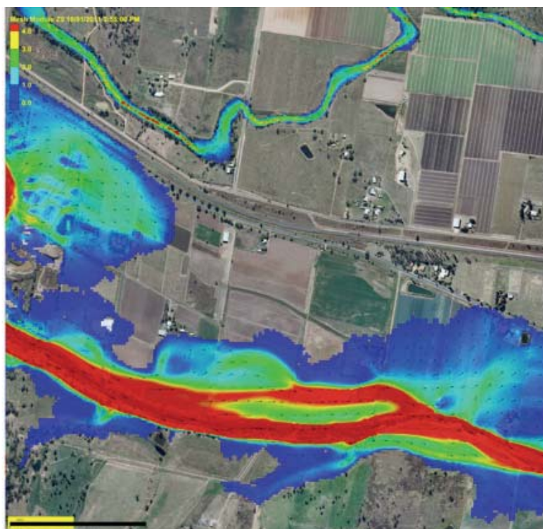
Figure 9.2 a to d – Chronology of Inundation, Western Grantham 3:25pm to 3:40pm (cont.)
