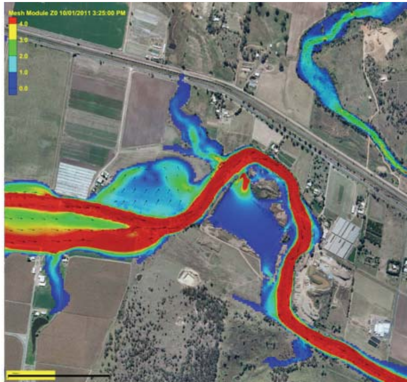
Figure 9.1 e to h – Chronology of Inundation, Quarry and Upstream 3:25pm to 3:40pm
