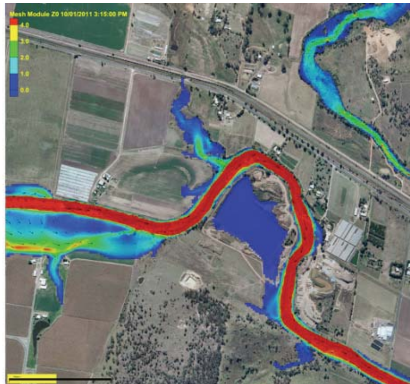
Figure 9.1 a to d – Chronology of Inundation, Quarry and Upstream 2:45pm to 3:20pm (cont.)
