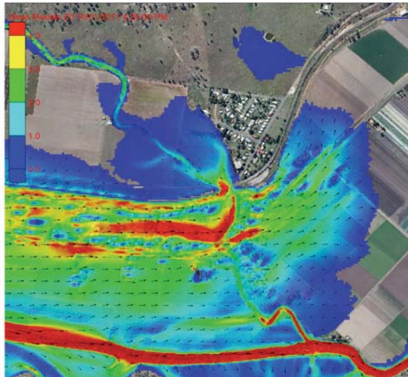
Figure 9.3 i to l – Chronology of Inundation, Eastern Grantham 4:25pm to 5:00pm
