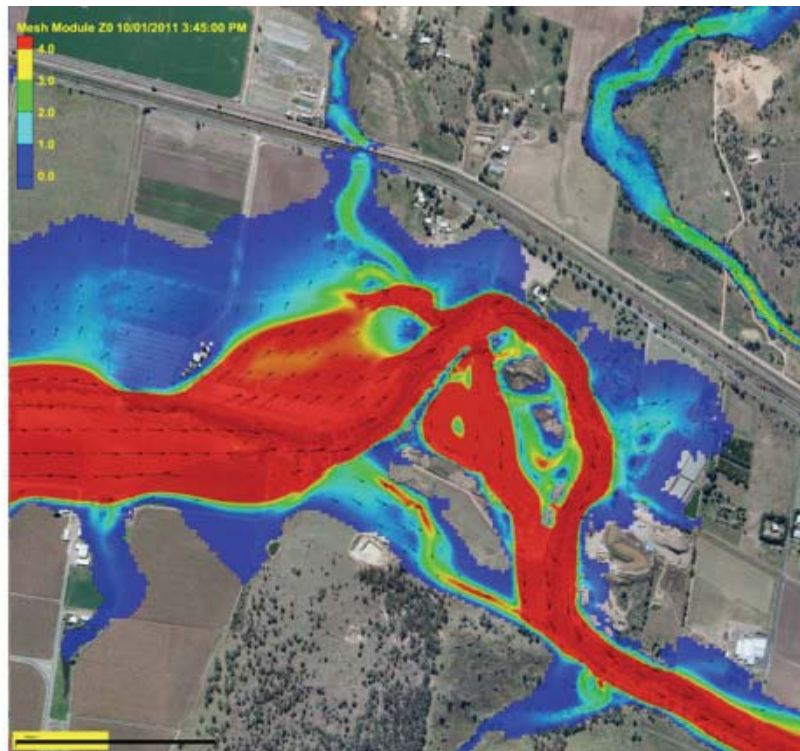
Figure 9.1 i to l – Chronology of Inundation, Quarry and Upstream 3:45pm to 4:20pm
