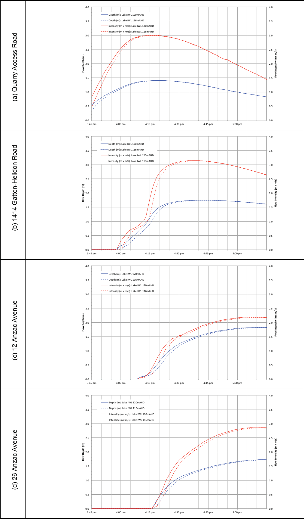
Figure 12.7 – Effect of Initial Lake Level on Flow Depth and Intensity
