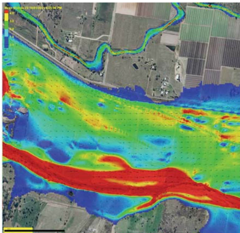
Figure 9.2 i to l – Chronology of Inundation, Western Grantham 4:25pm to 5:00pm
