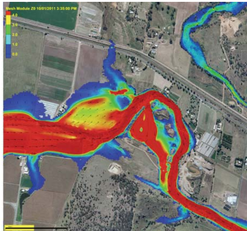
Figure 9.1 e to h – Chronology of Inundation, Quarry and Upstream 3:25pm to 3:40pm (cont.)
